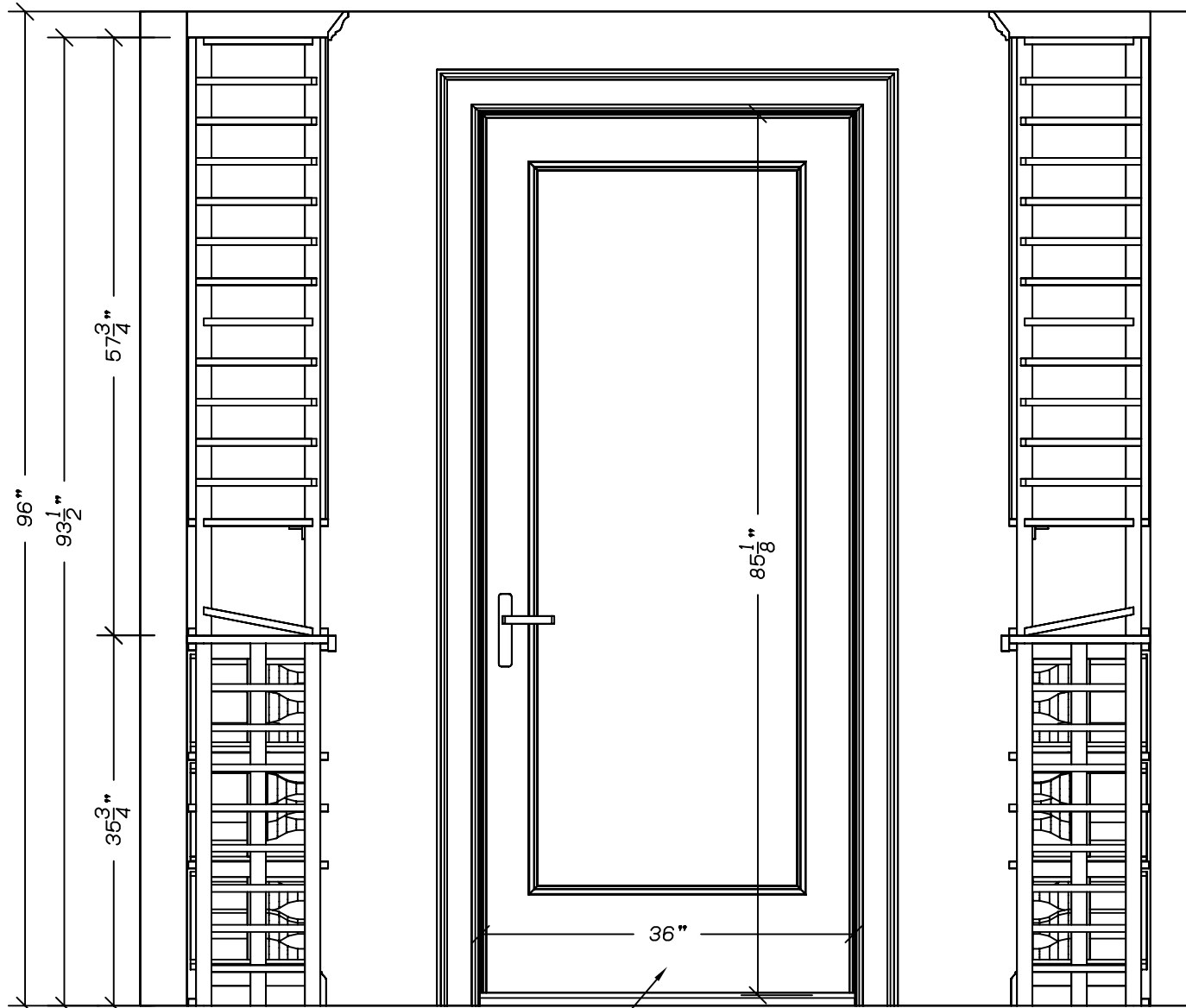
Single door (glass panel)
